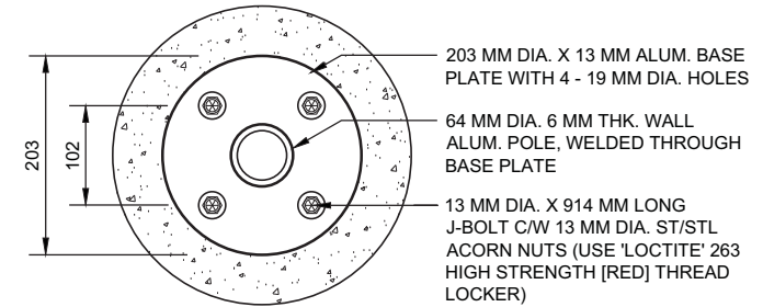
SECTION C
