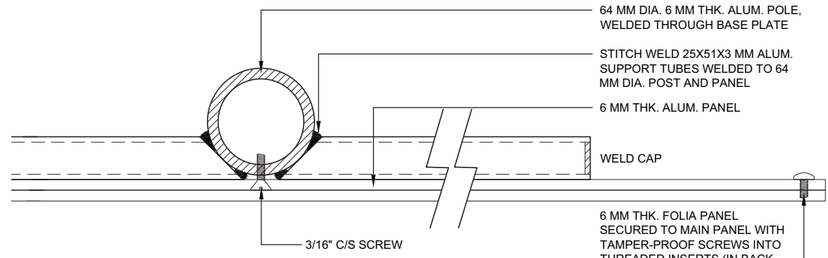
SECTION B
