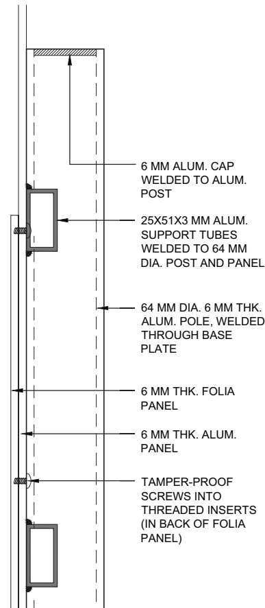
SECTION A
