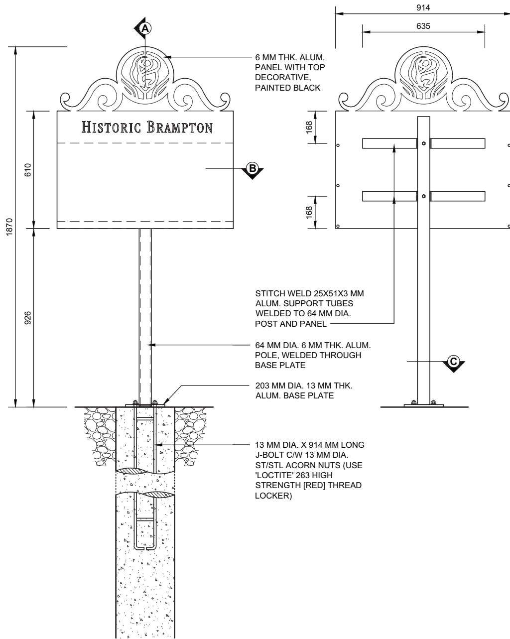
FRONT ELEVATION
